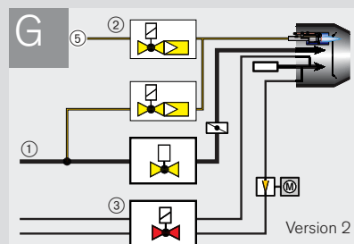
Dual-fuel: Gas and HFO ignition via main gas ignition burner with additional HFO ignition via LPG
