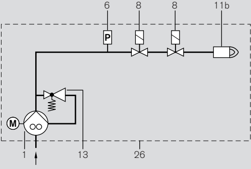
Gas oil ignition burner, WKMS 80
