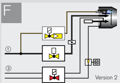
Dual-fuel: Gas and HFO ignition via main gas ignition burner
