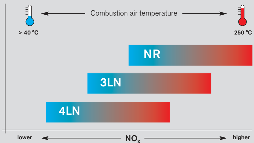
NO x emissions on hot-air WK-series burners, comparing NR and multiflam ® 3LN-version burners without flue gas recirculation and 4LN-version burners with flue gas recirculation
