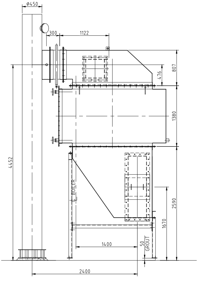
SECTION B SCALE 1:25
