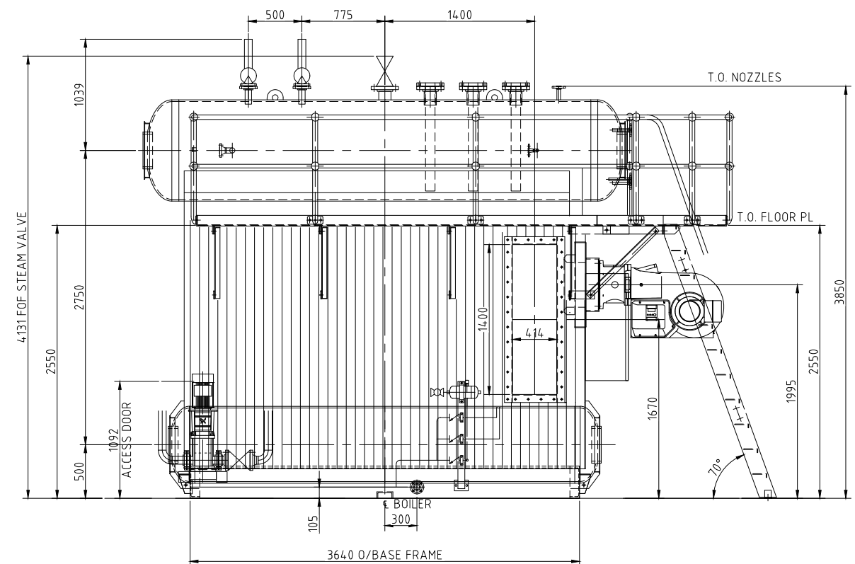
SECTION A SCALE 1:25
